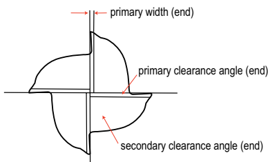
Non-Center Cutting End View
