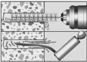
Clean dust from hole using a wire brush and pressurized air.
