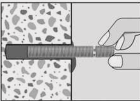
Insert anchor rod into hole with a slight twisting motion.
